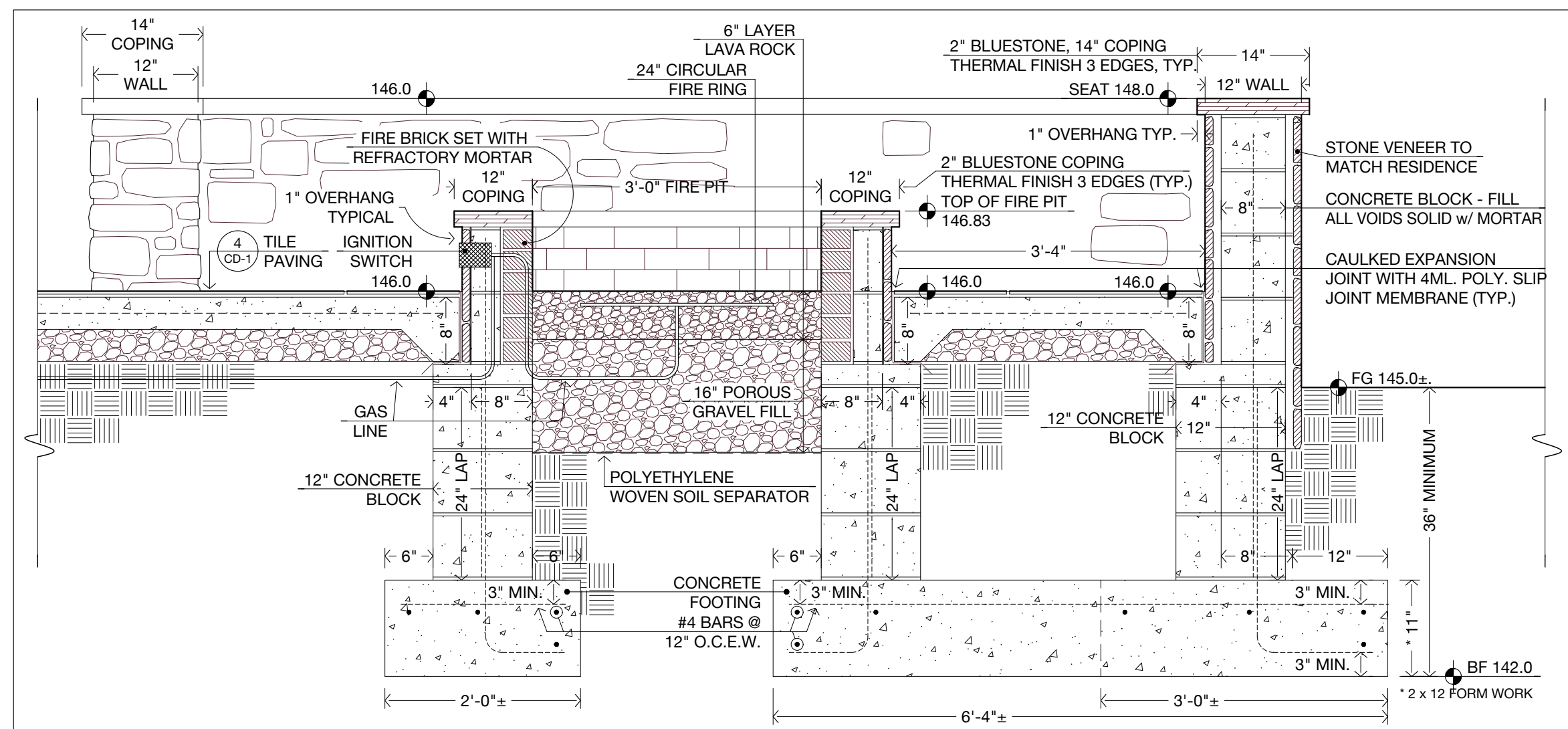
3 FIRE PIT SECTION 3/4" = 1'-0"
