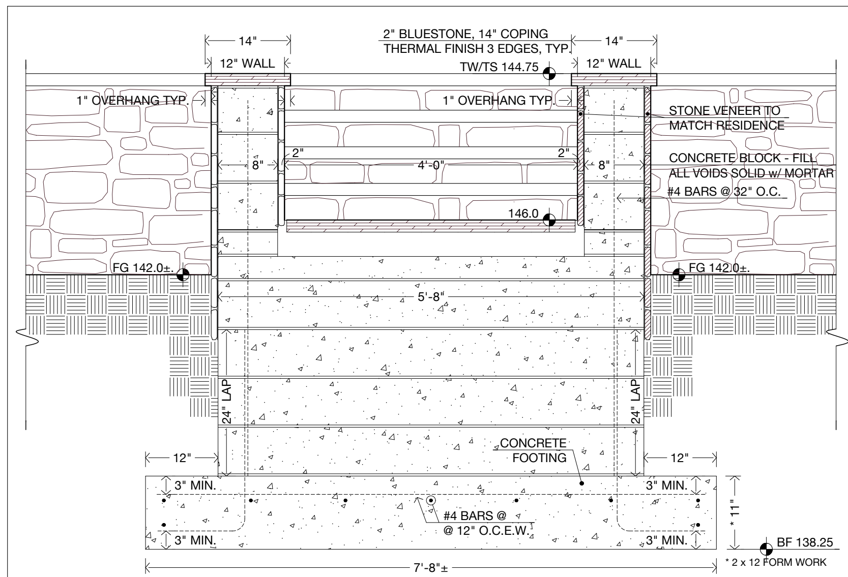
2 NORTH STAIR CROSS SECTION 3/4" = 1'-0"
