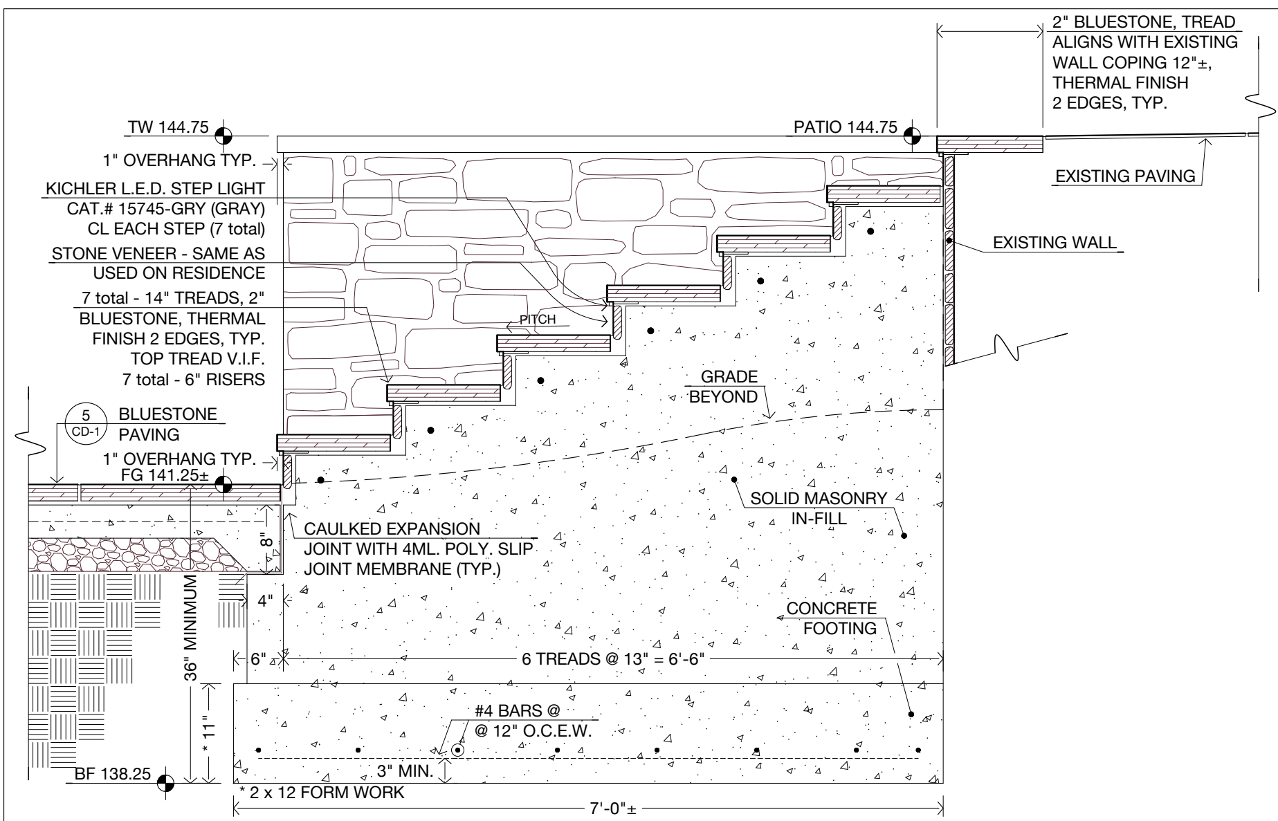
1 NORTH STAIR SECTION 3/4" = 1'-0"
